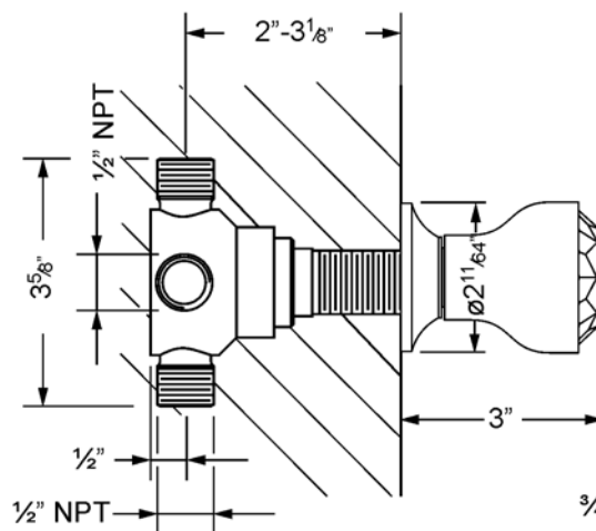
with concealed wall valve 649.40.620.000
